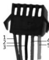
Controller Connector
